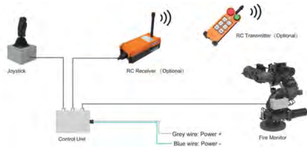
VMCS01 CONTROL SYSTEM WIRING
